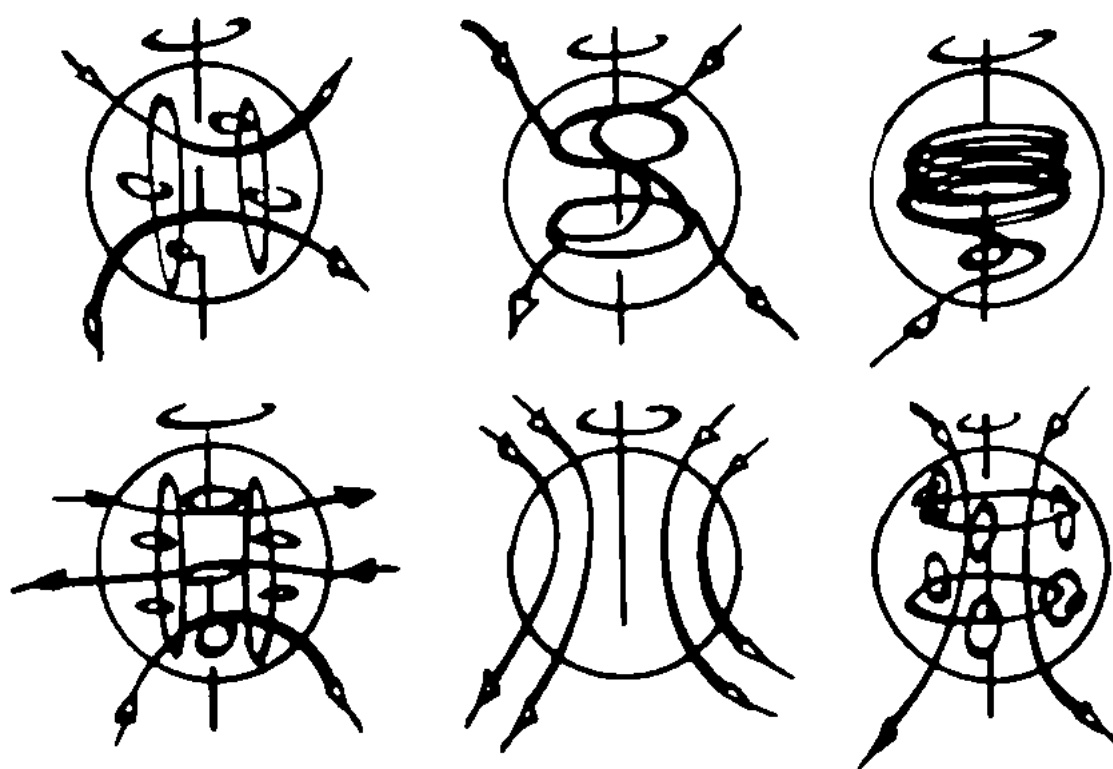
Fig. 26 The core's fluid motion, influenced by the Conors force, consists of a combination of differential rotation and convective turbulent helical motions. Neo-Sumenans considered such helical convolutions and spiralling dynamisms to be modes of radical participation between terrestrial entities and the Outside. Avoiding unification or convergence, these dynamisms suggested anomalous polytical movements (see Palaeopetrology: From Gog-Magog Axis to Petropunkism. on Trison and draco-spiraksm). Such spiral coils work through directional shear, intertwining communications, cataflights, synergetic oppositions and diffluence 10 between helical threads or communicating entities. The coils are usually characterized by development or intensification of a low-pressure center, a cosmodromk: cydone or singularity. Such spirals were frequently associated with the dynamism and distribution of Trisons or polytical units of the Middle East. Tiamaterialistic diagrams are manifestations of middle-eastern dracolatry (Zurvan Akarana, Tiamat, Azhi-dahaka, Apep and other coiling blasphemies). Parsani notes that Tiamatenalisbc movements were used by adept sorcerers or insurgents as blades for cutting through every manifestation of direction, appropriation and despotism (state, religion, survivalism, gravity, territorial forces, etc.): [They] are models of participation or alliances between the Earth and the Outside. The Middle East employs such models to be opened by the radical outsider rather than being open to the solar outside where thermonuclear capitalism reigns and planetary slavery awaits. The myth of Vitalism has not changed since the Dark Ages, the anthropomorphic earth as the center of the world has merely been cunningly replaced by Neo-Ptdemaic Heliocentrism. 'Sun at the center of our world' is the consequence of our submission to Solar Capitalism. Yet such submission is the price of believing in Solar Capitalism as the guarantor of eternal vitalism. Middle-eastern Tiamaterialism debunks the myth of Heliocentrism by awakening the Earth's insider and defying its politico-economic messengers and establishments on the planet.
